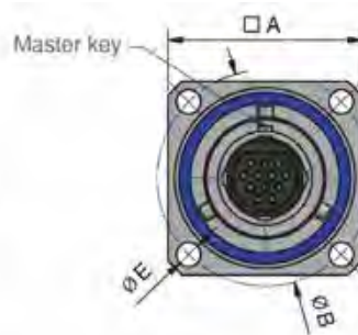
Rear mount square flange female PCB 0.075" pitch MCA3Bxxx-10S75Sxxx
