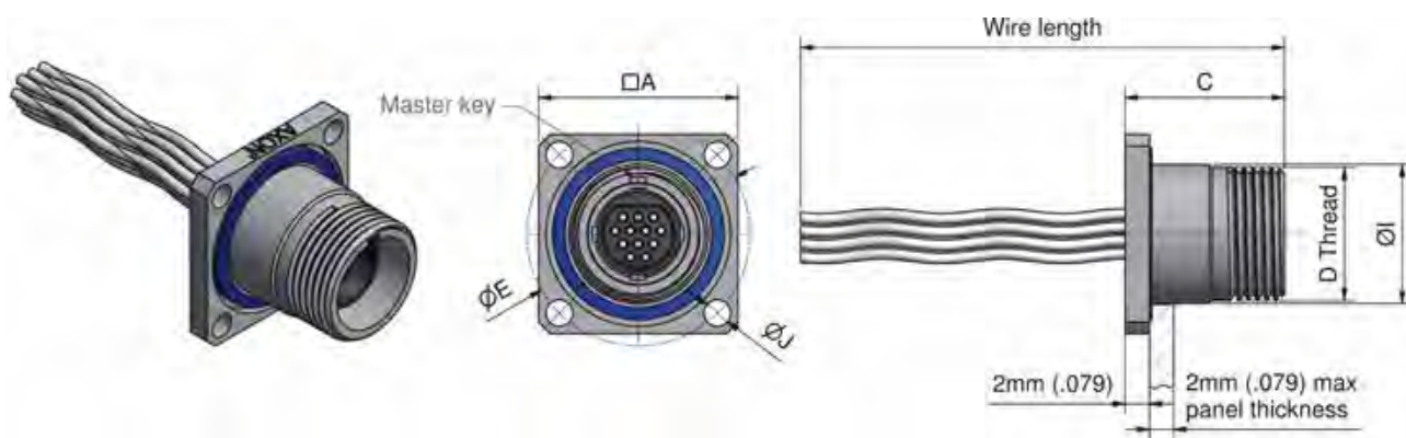
Rear mount square flange female MCATxxx-00Sxxxxxx
