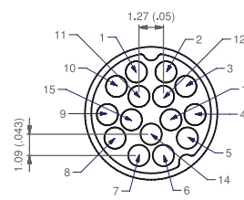
15 CONTACTS
