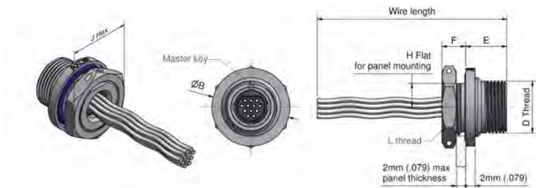
Front mount jam nut female MCATxxx-08Sxxxxxx
