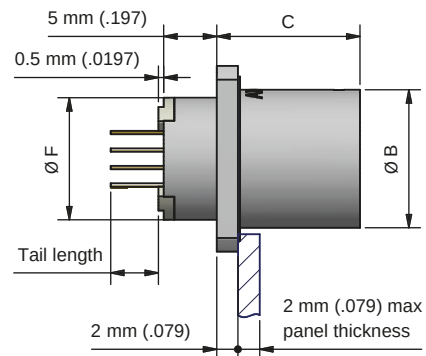
Rear mount square flange female PCB 0.075" pitch MCABKxxx-10S75Sxxx
