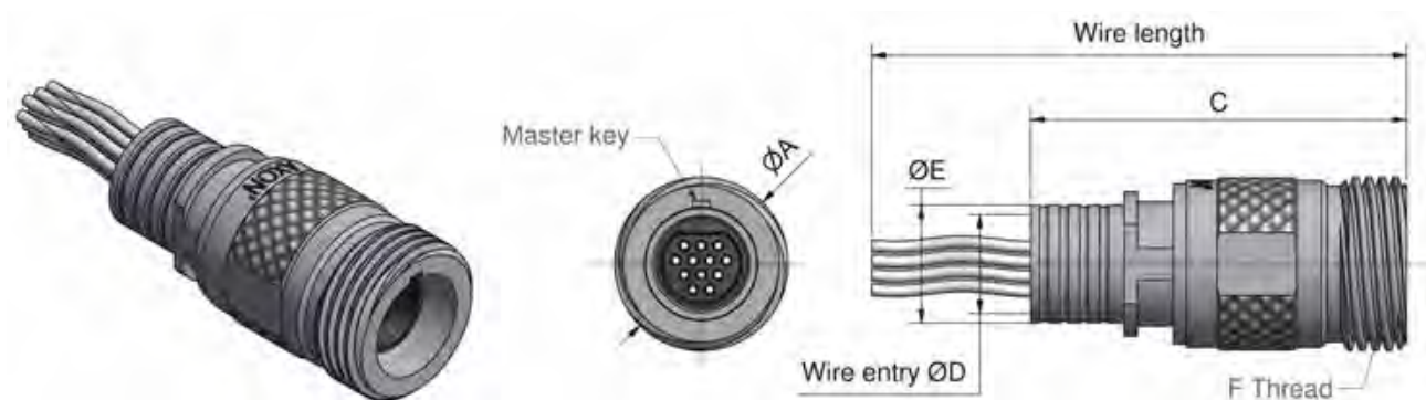
In-line female plug, screen termination funnel
