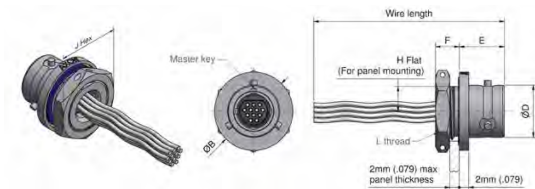
Front mount jam nut female MCA3Bxxx-08Sxxxxxx
