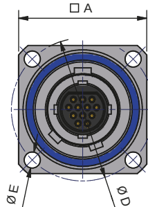
Rear mount square flange female PCB 0.050" pitch MCABKxxx-10S50Sxxx
