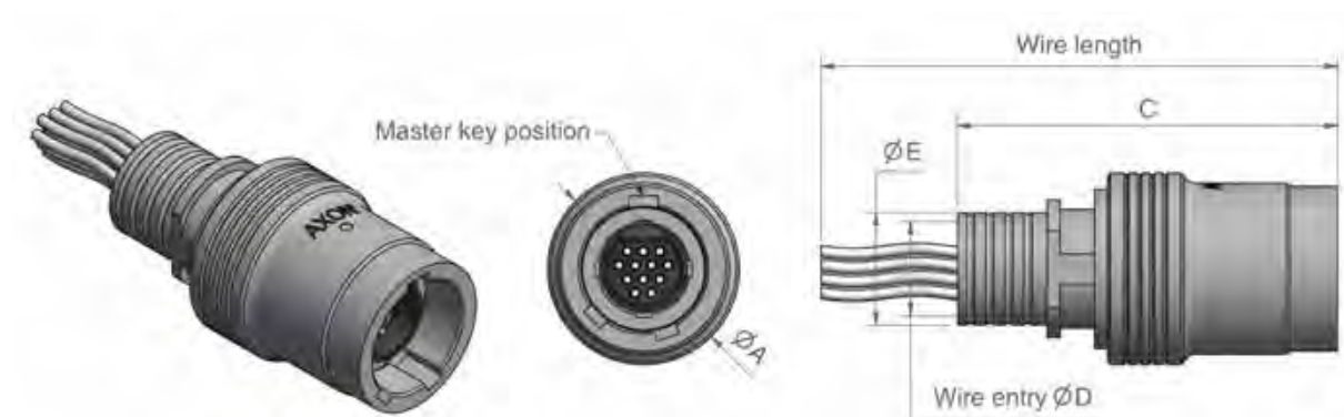
In-line female plug, screen termination funnel
