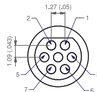
7 CONTACTS
