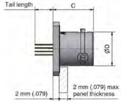
Rear mount square flange female PCB 0.050" pitch MCA3Bxxx-10S50Sxxx
